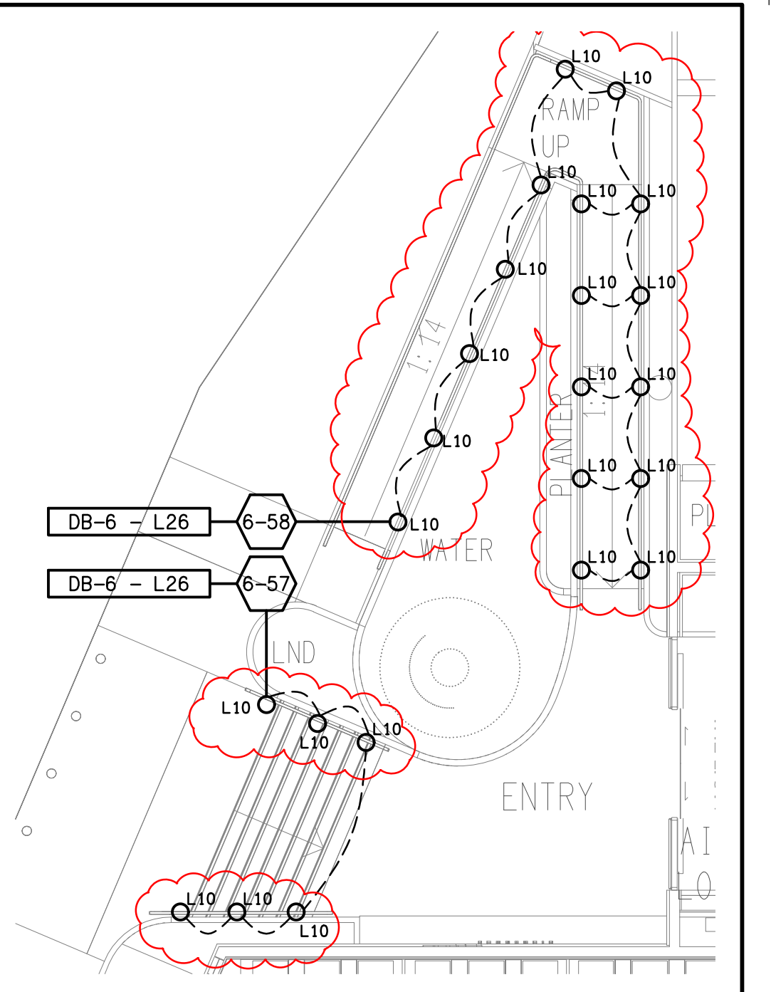
DETAIL HANDRAIL LIGHTING PLAN SCALE 1:100
